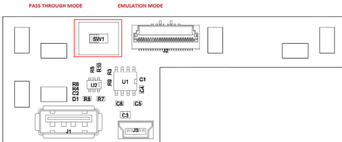
Figure 2.1: Clip-on PCB of Cobra ODE (with switch encircled).
